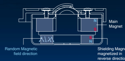
Conventional Tweeter Magnetic Circuit
