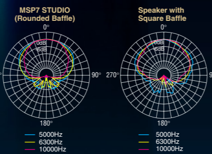
INTERNAL VS. EXTERNAL TWEETER MOUNTING
